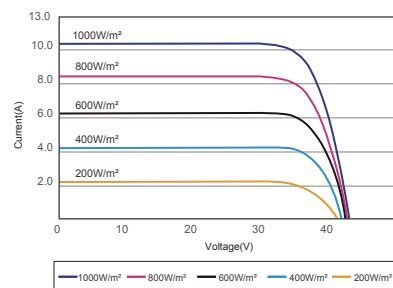
I-V Curves(530W)
