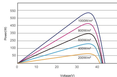
P-V Curves(530W)
